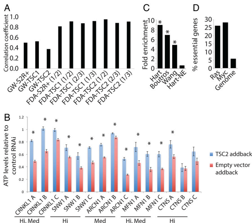
Fig. 1. SS/L interactions are enriched with essential genes. (A) Bar graph illustrating the correlation coefficients between pairs of replicates from the genome-wide (GW) or FDA screens as indicated. For the FDA screens, the numbers in parentheses indicate which replicates are compared in each case. (B) Bar graphs showing relative viability of TSC2 -deficient RA-derived cells with either TSC2 cDNA (blue bars) or empty vector (red bars) addback transfected with the indicated shRNA constructs relative to control shRNA transfection, measured using CellTiter-glo assays. Bars represent average values from nine replicates in each case, and error bars indicate SEM. Asterisks indicate cases where viability of empty vector addback samples is significantly lower than TSC2 cDNA addback samples ( P < 0.05 ) as determined using t tests. The confidence class with which each gene was identified in the genome-wide screen is indicated below the gene names (Hi, high confidence; Med, medium confidence). (C) Bar graph showing fold enrichment of essential genes among SS/L genes identified from the genome-wide screen. Three independent datasets were used to define essential (19, 20, 21) or nonessential genes [Hart-NE (20)]. Asterisks indicate statistically significant enrichment ( P < 0.05 ) based on Z-tests to compare with 1,000 permutations of randomly selected genes. (D) Bar graph illustrating the percentage of genes identified as SS/L with Ras or Myc overexpression or activation in previous studies. "Genome" indicates the percentage of essential genes in the whole genome assessed using the same datasets as in C combined to define essential genes (19, 20, 21).
