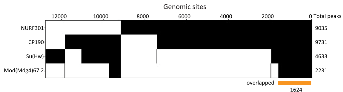
Figure 3. NURF301 interacts physically with gypsy insulator proteins, and these factors co-localize genome-wide. (A) Co-immunoprecipitation of NURF301 with core gypsy components. Nuclear extracts (NE) are from embryos aged 0–24 h collected at RT, which is the same material used for IP followed by mass spectrometry. NE was immunoprecipitated with each antibody or with normal serum (IgG) as indicated. Unbound supernatant (Sup) and bound (IP) fractions are also shown. Polycomb (Pc) is used as a negative control. (B) Representative screenshot of ChIP-seq profiles shows NURF301 co-localizes extensively with gypsy core components in Kc cells grown at 25°C. Peaks called by MACS2 are indicated by black bars. Three biological replicates were examined for each sample. (C) Binary heatmap of CP190, NURF301, Su(Hw), and Mod(mdg4)67.2 binding sites in Kc cells, ordered by supervised hierarchical clustering. Each column represents a single independent genomic location, and a mark in a row indicates presence of the indicated factor. Total peaks of each factor are shown on the right. 7423 genomic sites co-localize between NURF301 and CP190, and 1624 genomic sites (yellow bar) were bound by all four factors. (D) Average signals of CP190 and NURF301 peaks, but not of Su(Hw) and Mod(mdg4)67.2, accumulate at the TSS.
