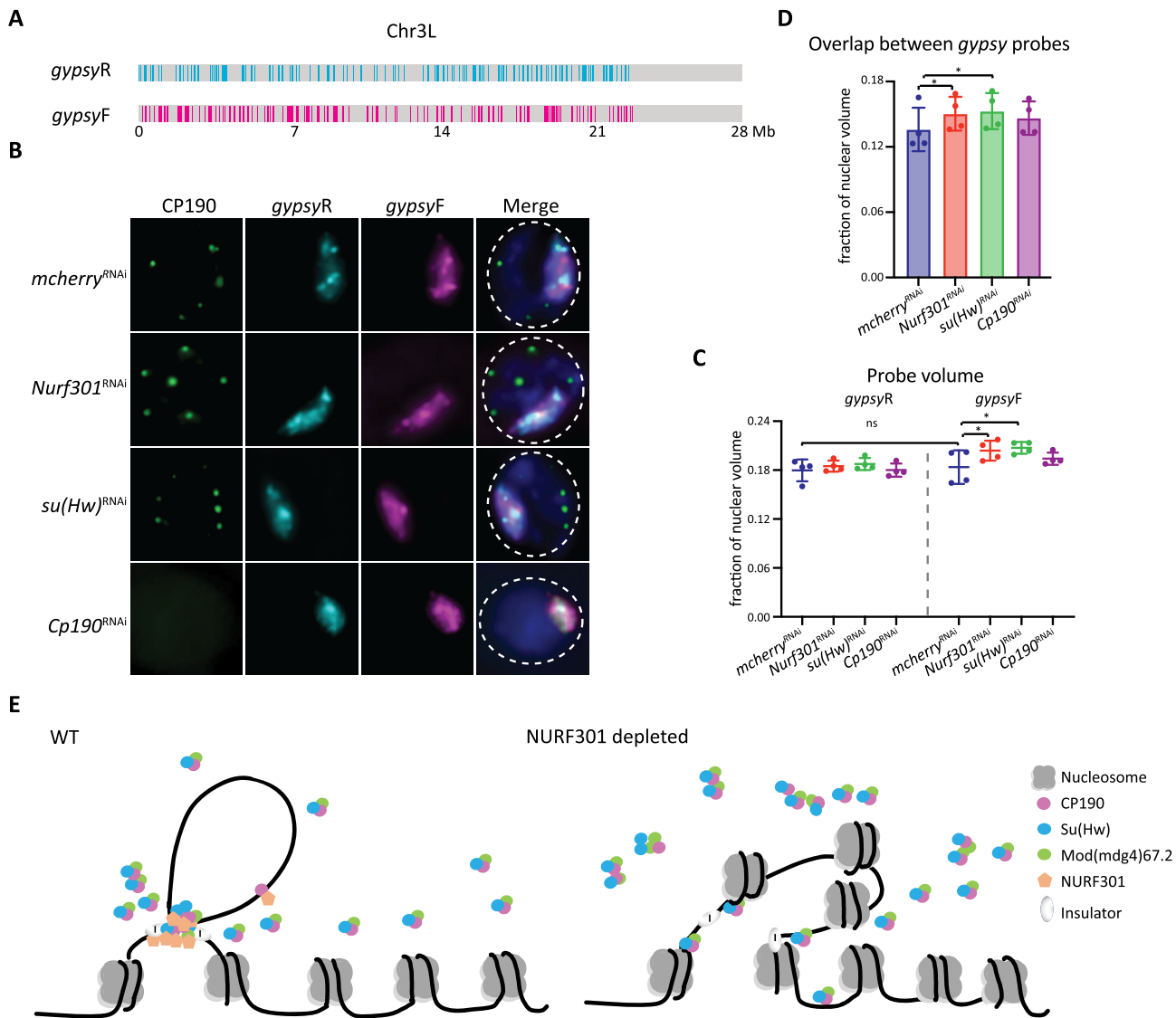
Figure 7. Depletion of NURF301 specifically alters 3D arrangement of gypsy insulator binding sites. (A) Schematic of gypsy probes on Chr3L. The co-occupied sites of Su(Hw)/CP190/Mod(mdg4)67.2 are designated as gypsyF probe, and the 1D reverse of non- gypsy sites are designated as control probe ( gypsyR ). The DNA amount labeled by gypsyF or gypsyR paint is ~5 Mb. (B) Representative images of CP190 IF and signals of gypsyF and gypsyR probes in dsRNA treated Kc cells. Cells were cultured at 25°C. Images are maximal projections of 26 Z-stacks. Nuclear edge is indicated with dashed line. Scale bar: 2 \mu m. (C) Probe volume relative to the fraction of nuclear volume. Left panel is control gypsyR probe, right is gypsyF probe. (D) Intermixing volume of gypsyF and gypsyR paints relative to nuclear volume. Data are from four biological replicates and a dot represents each replicate, n > 300 cells in each sample. Paired t-test was used, and error bars show standard deviation. ns, not significant; * P < 0.05 as indicated. (E) Nucleosome remodeller NURF301 cooperates with Su(Hw) to promote stable insulator complex binding at gypsy insulator sites to establish higher-order chromatin structure. After depletion of NURF301, Su(Hw) and CP190 cannot properly bind to gypsy binding sites, thus impairing gypsy insulator function and influencing chromatin organization.
